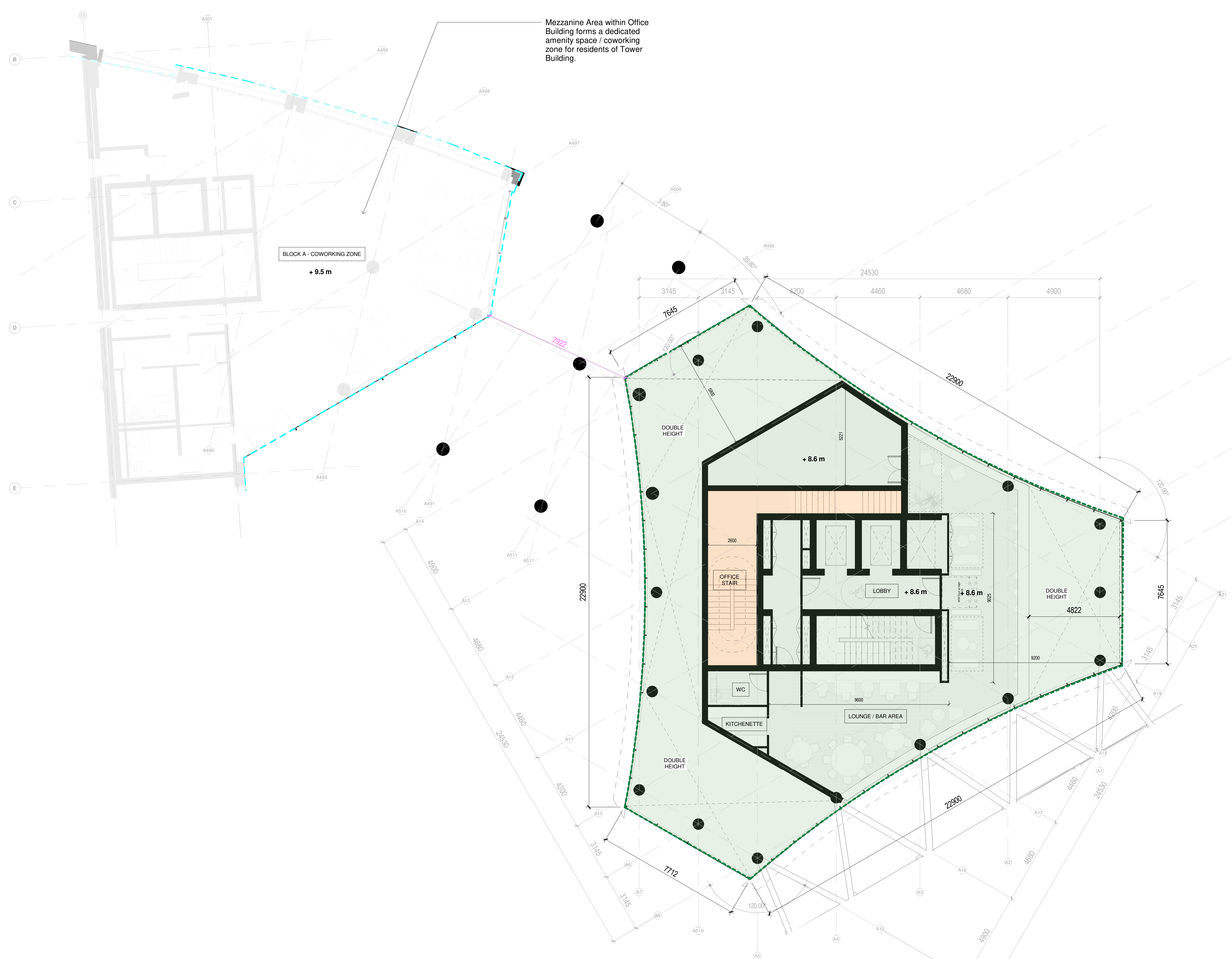
Proposed Mezzanine Floor Plan - Tower 1 : 100
